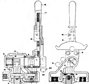
Figs. 2481-2482. 3/4-Inch Straight-Air Engineer's Brake Valve.
